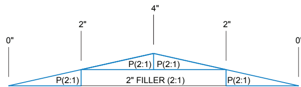
(A) DETAIL
